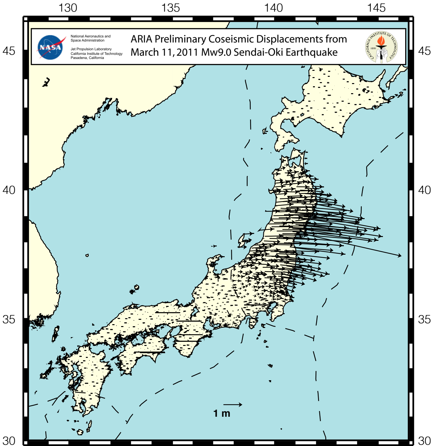
Figure shows horizontal displacements based on estimated position of GEONET stations at 06:00 UTC on March 11, using JPL's Rapid orbit solution and using JPL's GIPSY-OASIS software. Bars at end of vector show 95% error estimate. Solutions courtesy of ARIA team at JPL and Caltech. All original GEONET RINEX data provided to Caltech by the Geospatial Information Authority (GSI) of Japan.
