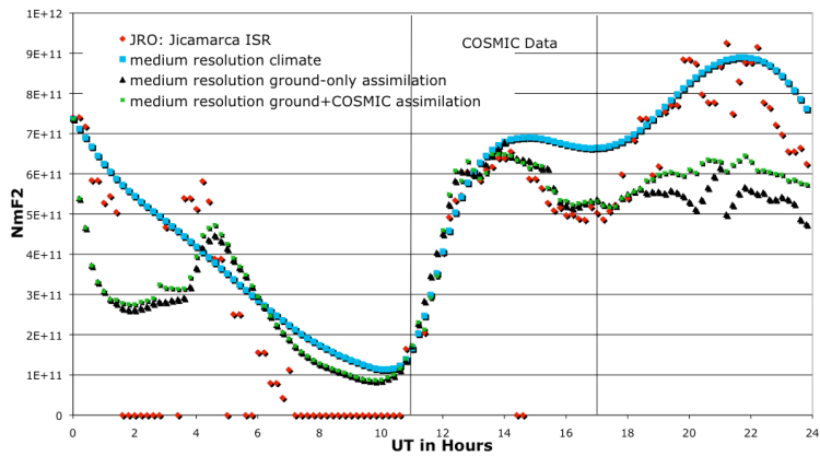
GAIM Medium Resolution Assimilation Results for Sept 21, 2006
