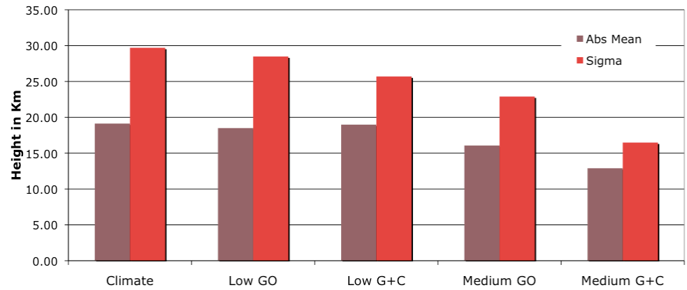
HmF2 Comparison of Low and Medium Resolution Runs for Sept 21, 2006
