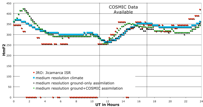
GAIM Medium Resolution Assimilation Results for HmF2 on Sept 21, 2006
