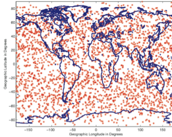
COSMIC Data Occultations on a Typical Day: Each Marker Represent a Separate Occultation
