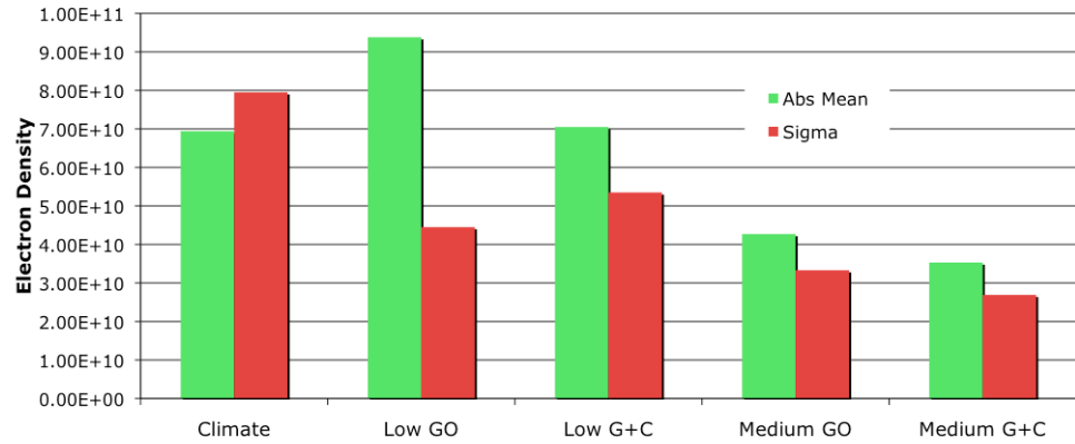
NmF2 Comparison of Low and Medium Resolution Runs for Sept 21, 2006
