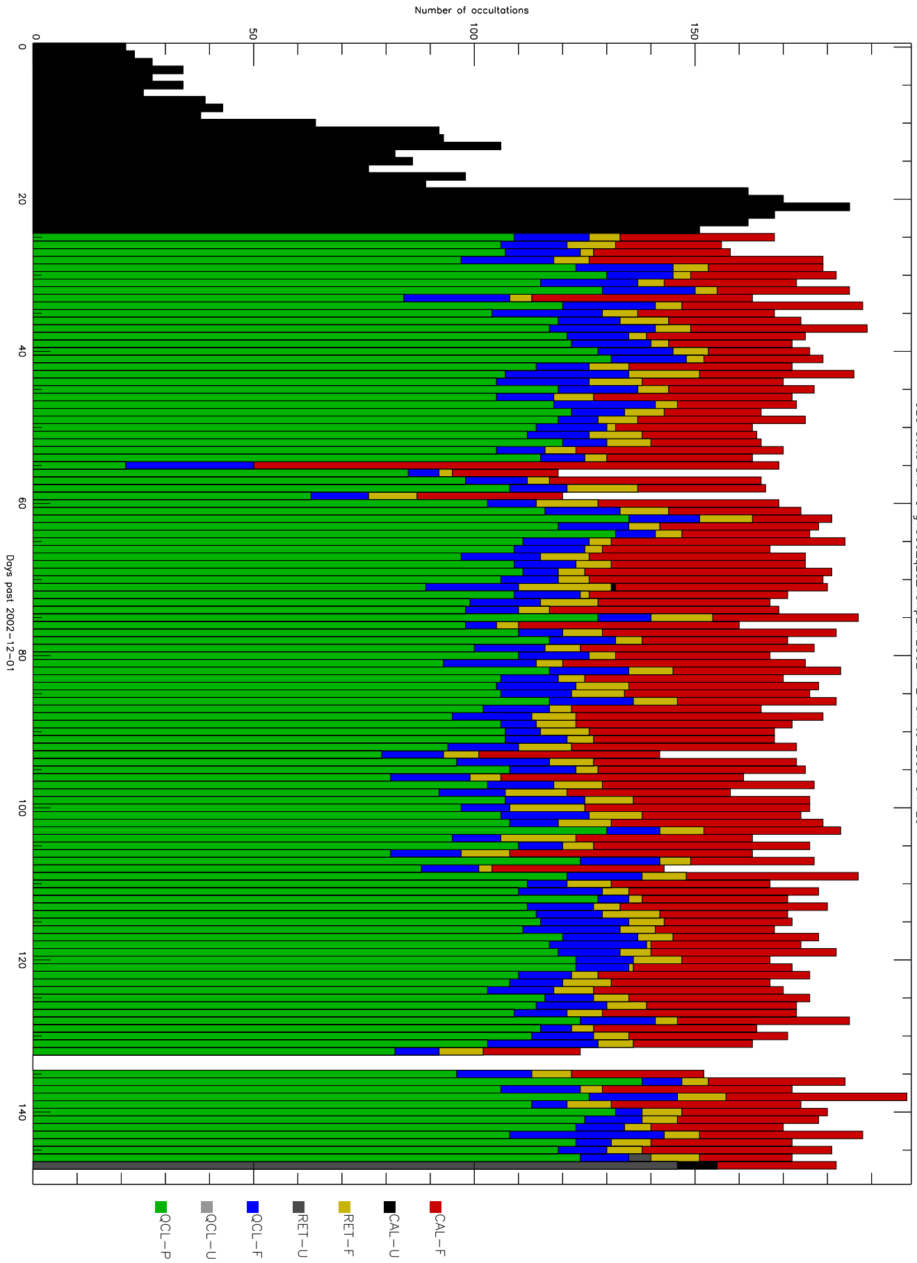
GEO stats SAC-C q150o-q2s-10kp2N 2002-12-01 to 2003-04-29
