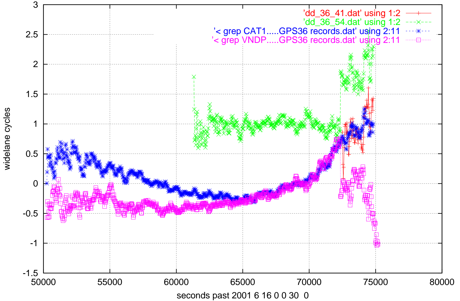
Double differenced widelanes for CAT1-VNDP
